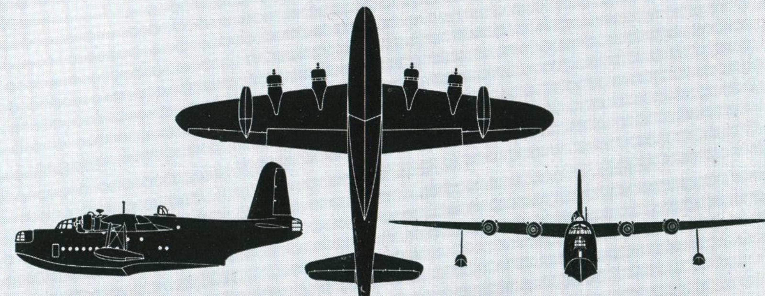
Short SUNDERLAND GR Mk.5 (Four P & W Twin Wasp radial) Span : 112 ft. 9 in. Length : 85 ft. 4 in.
