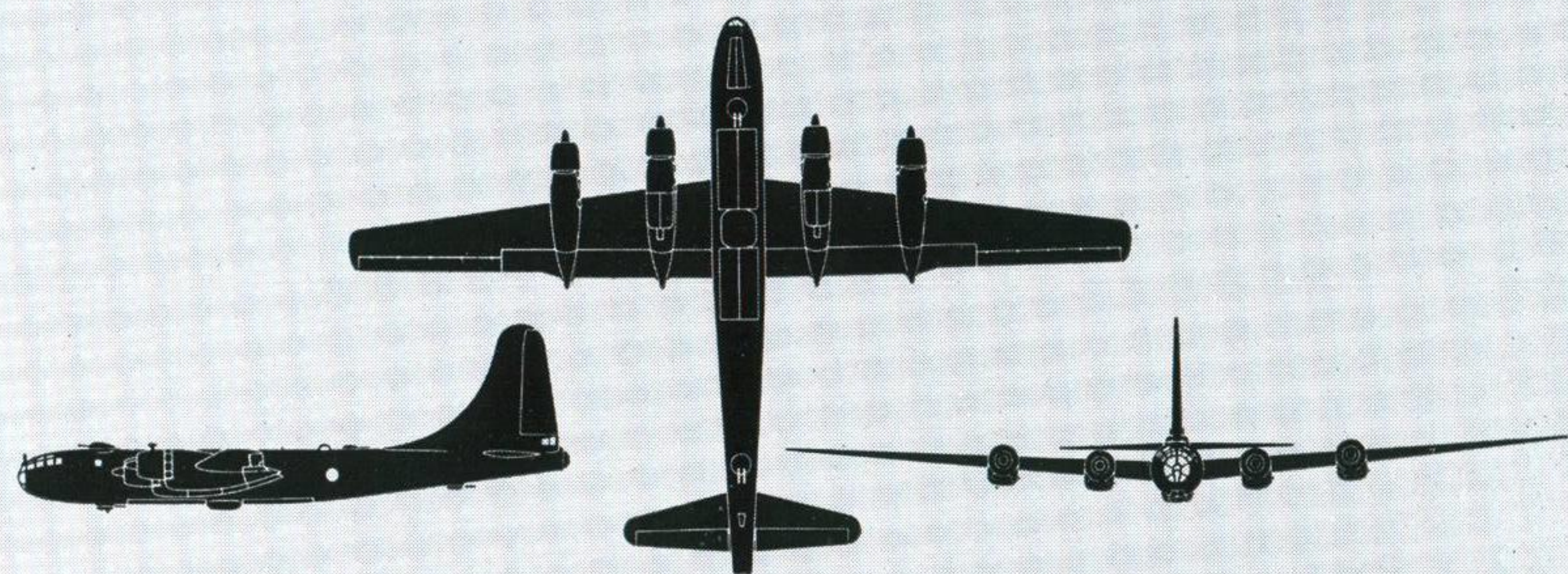
Boeing SUPERFORTRESS USAF : B-50A (Four P & W Wasp Major radial) Span : 141 ft. 3 in. Length : 99 ft.
