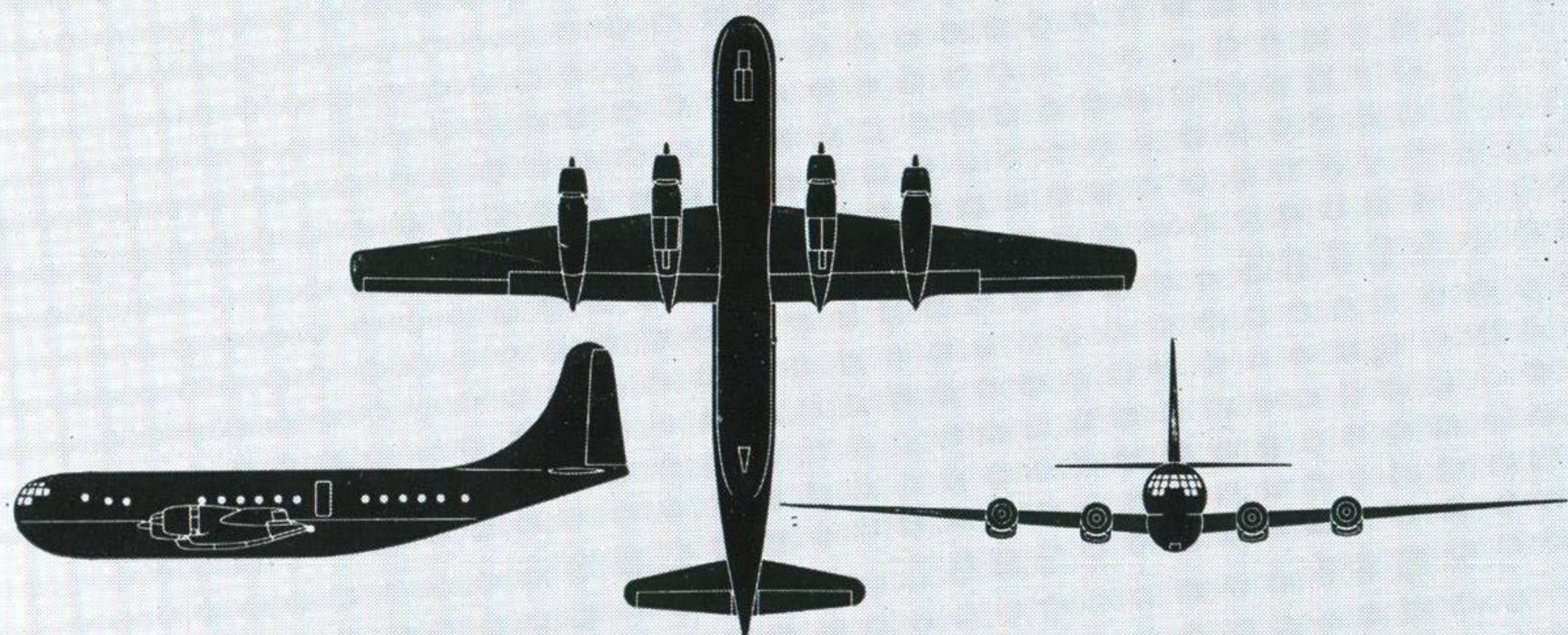
Boeing STRATOCRUISER USAF : C-97 (Four P & W Wasp Major radial) Span : 141 ft. 3 in. Length : 110 ft. 4 in.
