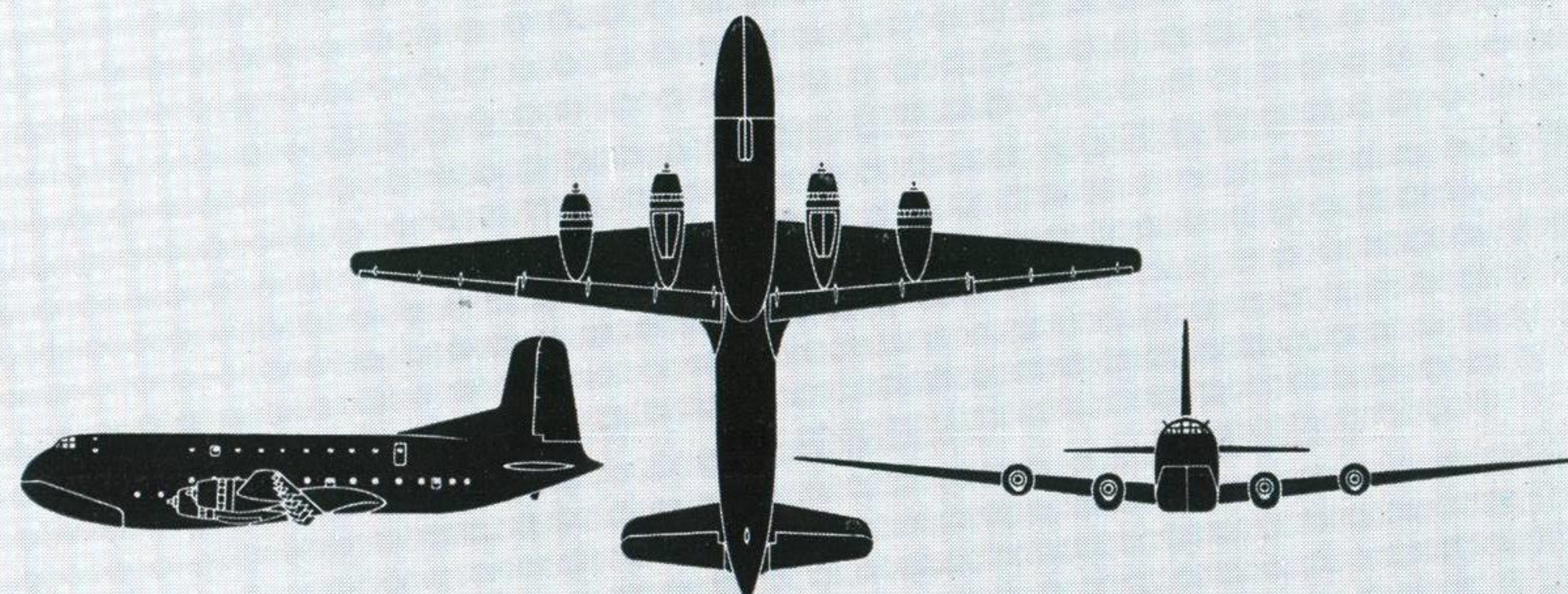
Douglas GLOBEMASTER 2 USAF : C-124A (Four P & W Wasp Major radial) Span : 173 ft. 3 in. Length : 127 ft. 2 in.
