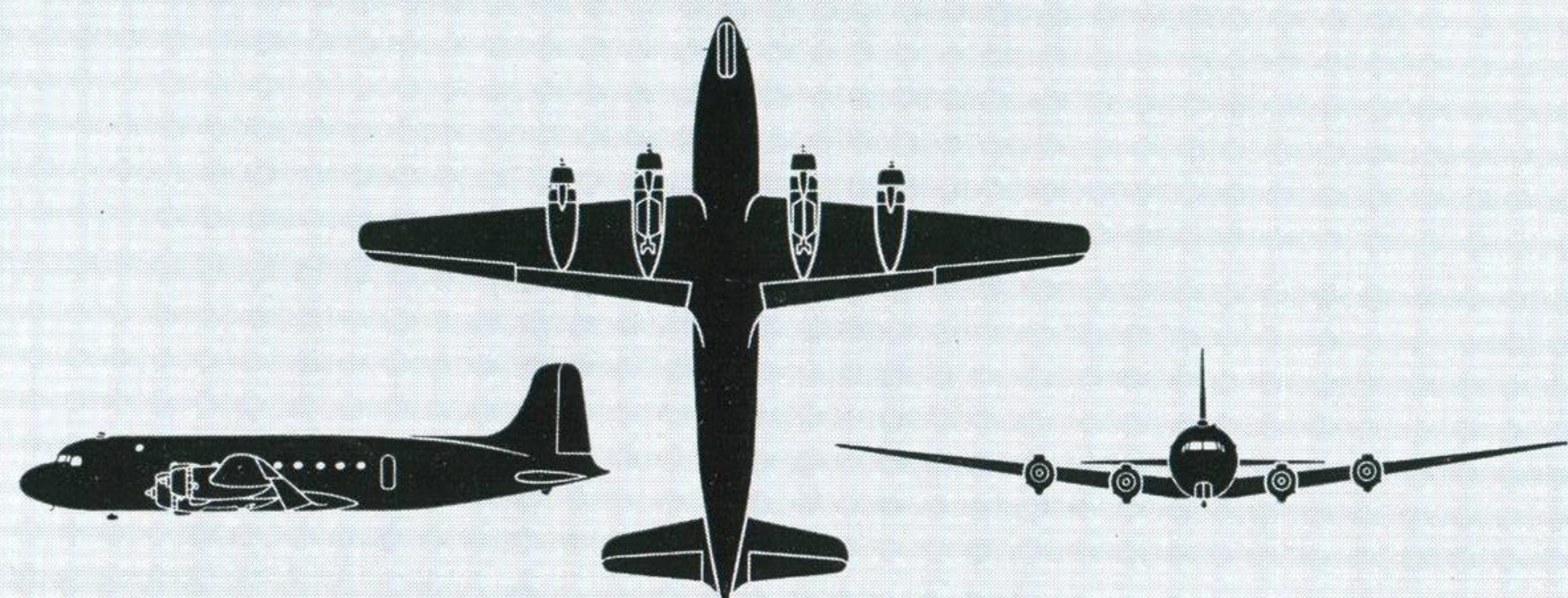
Douglas SKYMASTER (DC-4) USAF : C-54 (Four P & W Twin Wasp radial) Span : 117 ft. 6 in. Length : 93 ft. 11 in.
