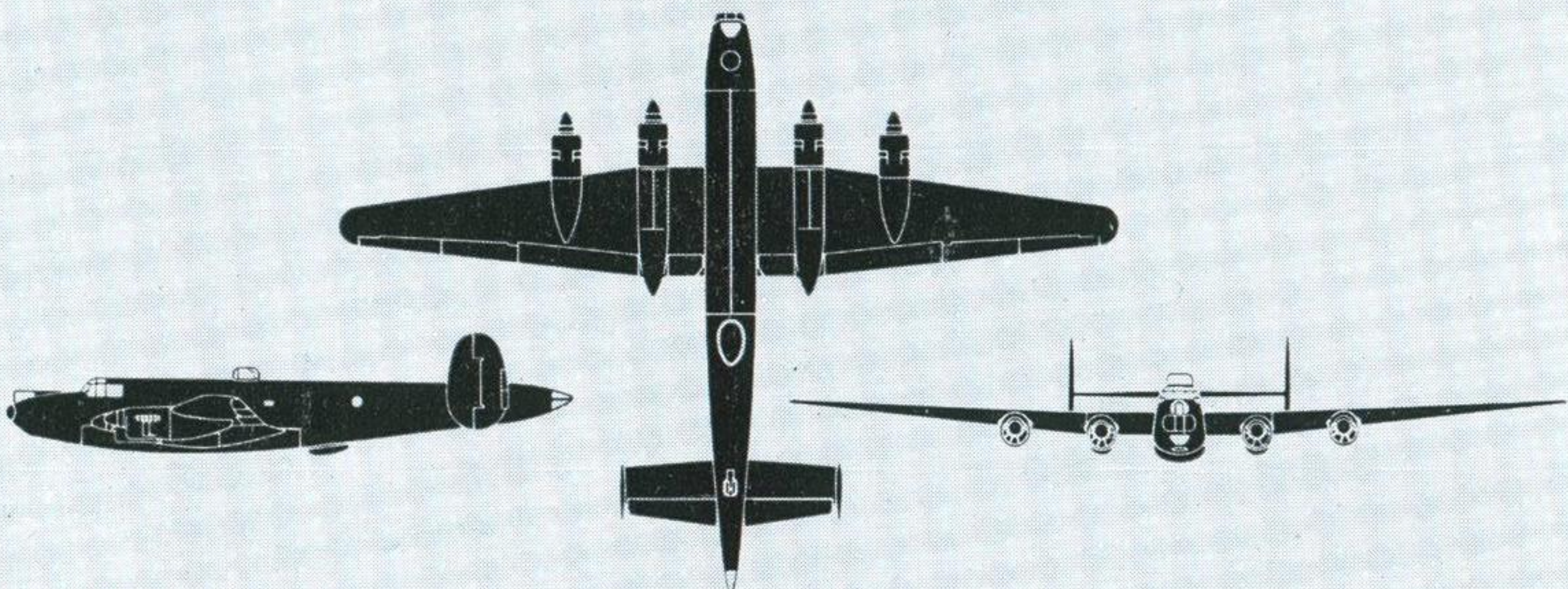
Avro SHACKLETON MR Mk.2 (Four R.R. Griffon radial) Span : 120 ft. Length : 87 ft. 3 in.
