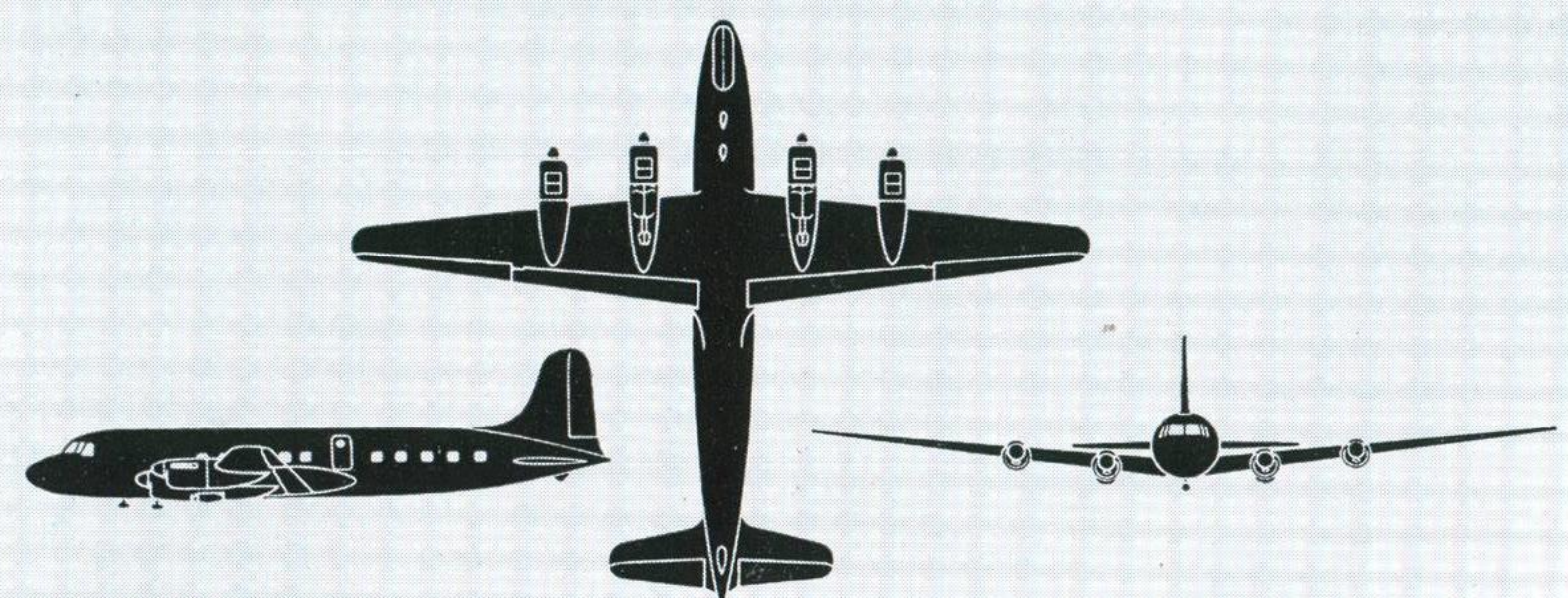
Canadair ARGONAUT (C-4) (Four R.R. Merlin radial) Span : 117 ft. 6 in. Length : 93 ft. 7 in.
