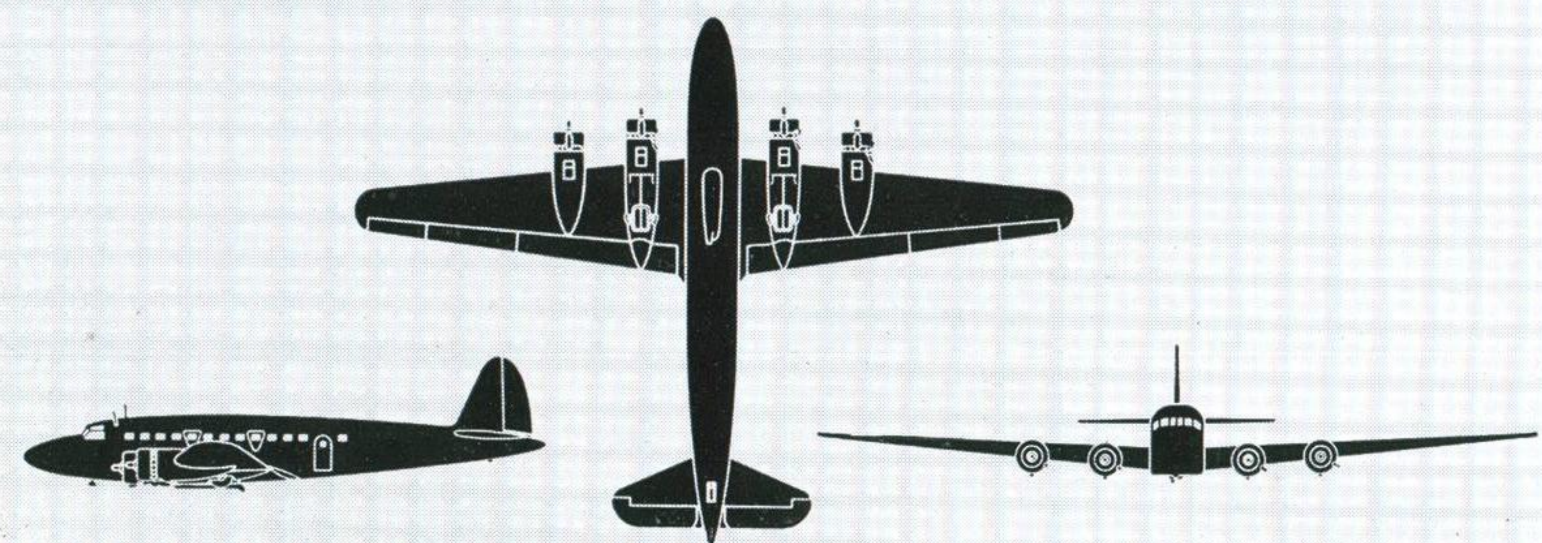
Siai-Marchetti SM.95 (Four P & W Twin Wasp radial) Span : 112 ft. 5 in. Length : 81 ft. 3 in.
