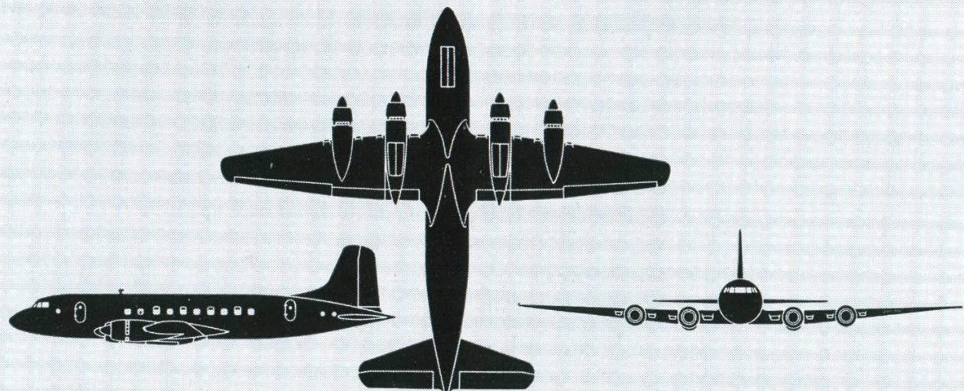
Handley Page HERMES Mk. 4 (Four Bristol Hercules 763 radial) Span : 113 ft. Length : 96 ft. 10 in.
