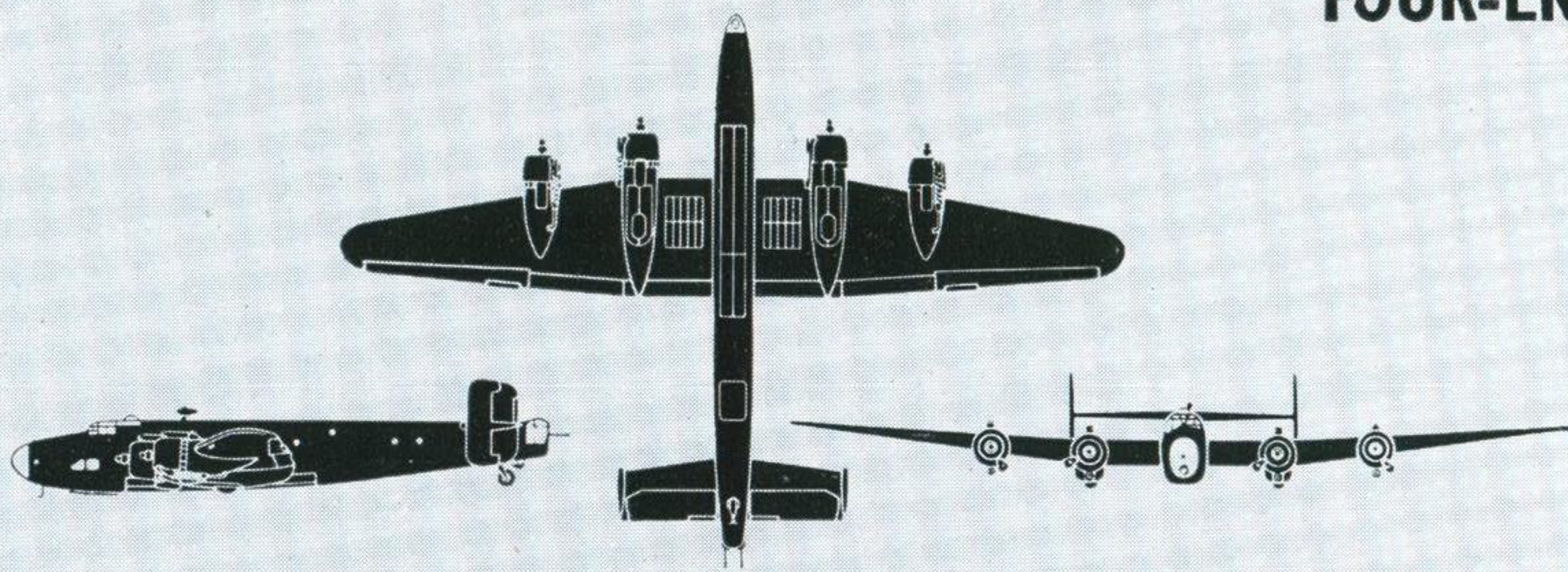
Handley Page HALIFAX A Mk. 9 (Four Bristol Hercules radial) Span : 104 ft. Length : 73 ft. 7 in.
