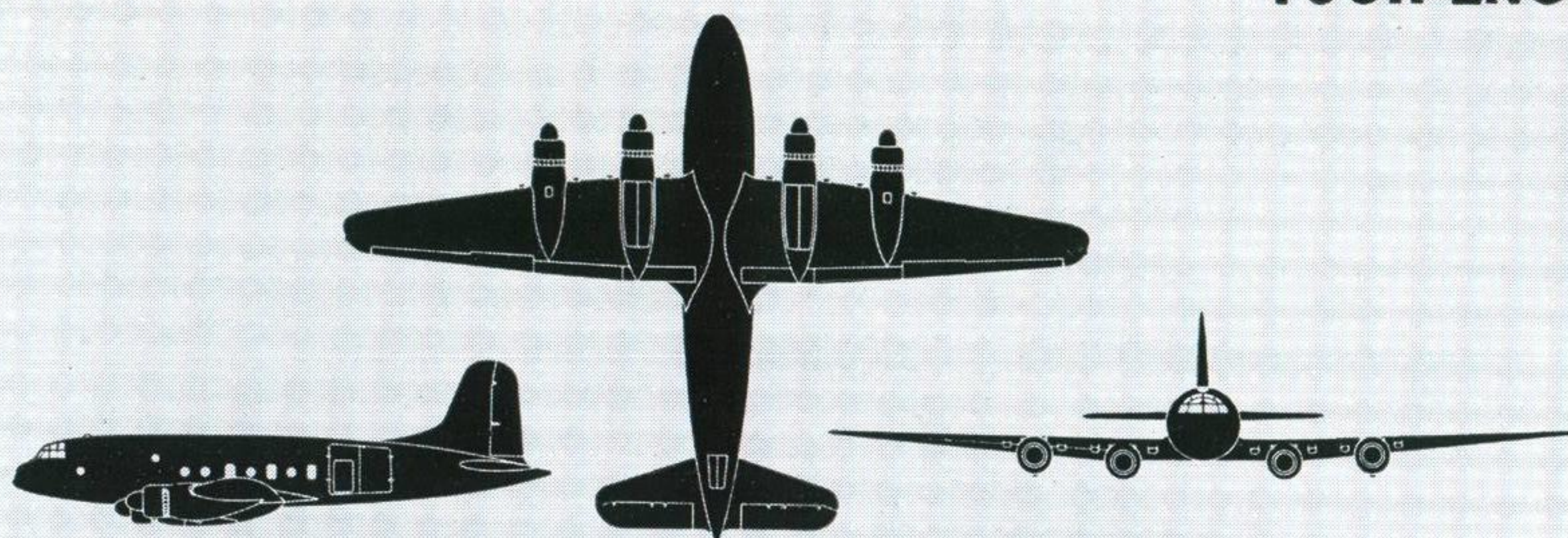
Handley Page HASTINGS C Mk. 1 (Four Bristol Hercules 101 radial) Span : 113 ft. Length : 81 ft. 8 in.
