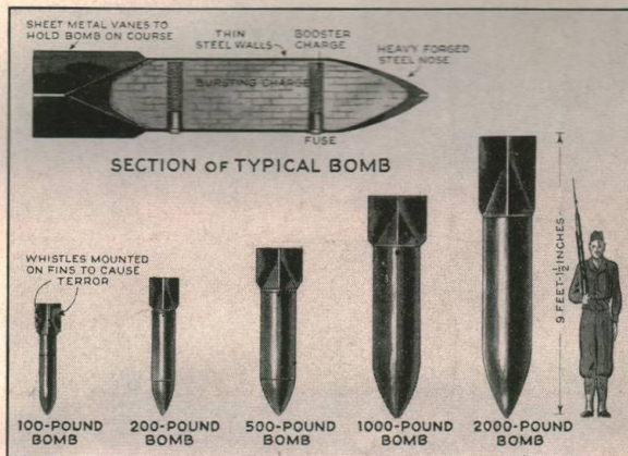
CATALOG OF GERMAN BOMBS SHOWS THEIR SIZE AND CONSTRUCTION
