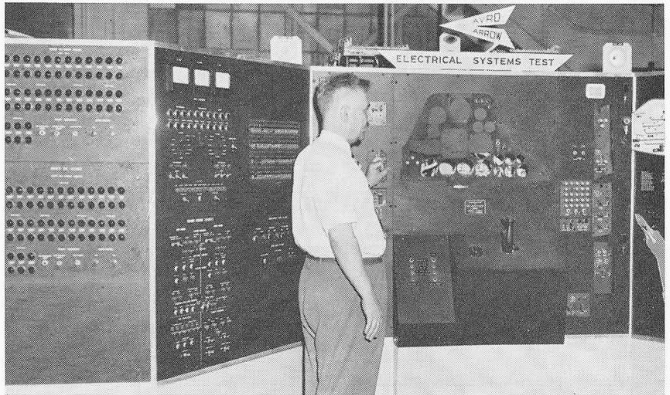
Arrow electrical system test rig simulates exactly the complete electrical system in the aircraft. Any production electrical component can be easily checked for serviceability in the test rig.
