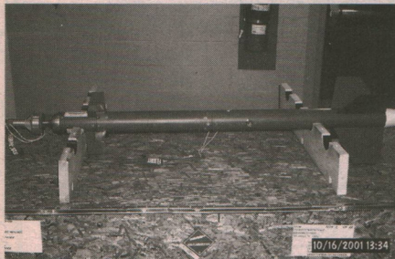
Fin Assembly MXU 651 complete with inner packaging. (The fins are assembled to the bomb body)
