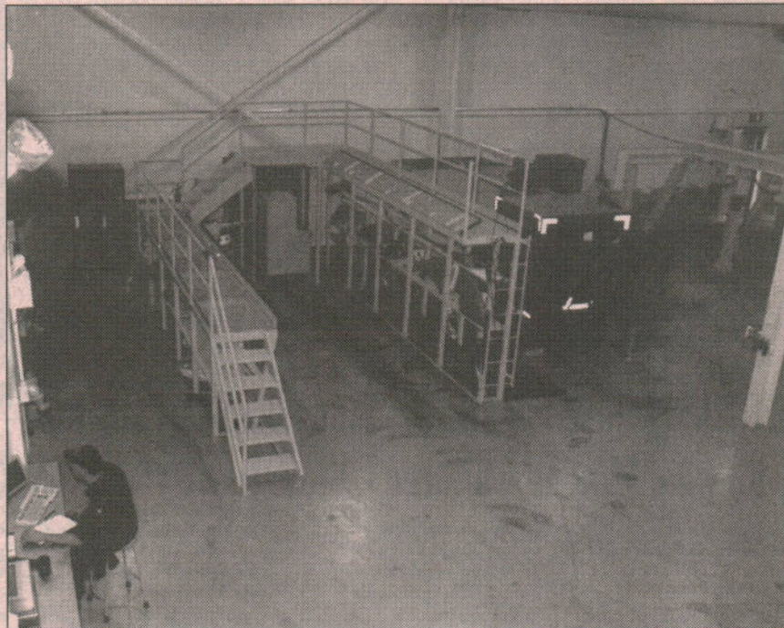
New AAR Fuselage Tank Repair Stand
