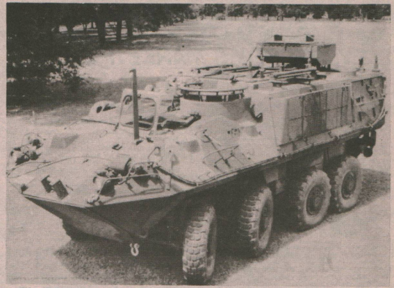
The BISON, and APC produced in Canada and bought especially for the Militia, will be making its first appearance at MILCON 91. Different versions of this vehicle form a major component of the U.S. Marine Corps mechanized fleet.
