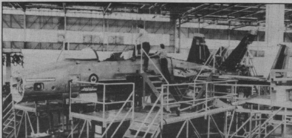
IN PRODUCTION — The first of 138 CF-18 Hornet tactical fighters for the Canadian Forces undergoes final assembly at McDonnell Douglas Corporation facilities in St. Louis. Canada selected the multimission, twin-engined Hornet in March 1980 to replace its CF-101, CF-104 and CF-5 aircraft. Delivery of the first CF-18 is slated for October, and deliveries at a rate of two aircraft per month will extend to 1988.
