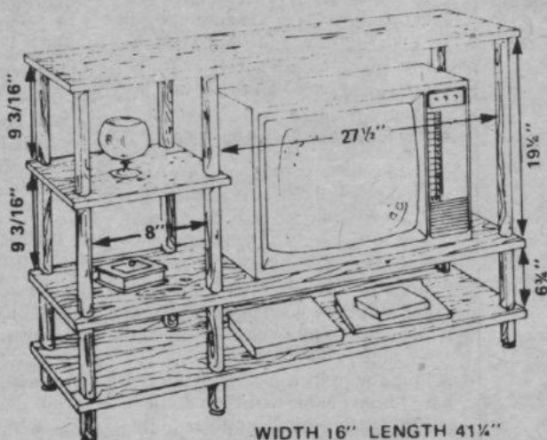
WIDTH 16" LENGTH 41 1/4" HEIGHT 31 1/2"
