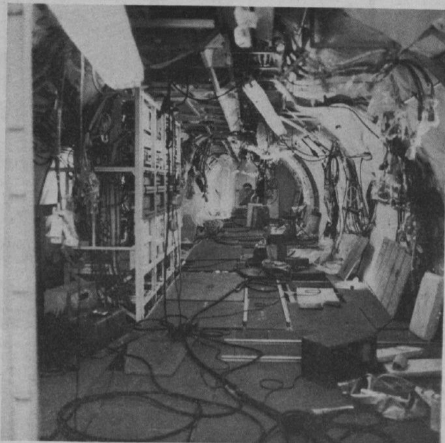
An interior view of the fuselage; taken on Oct 17th from the forward bulkhead looking aft. On the left the Main Electrical Load Centre has been installed while the wire harnesses hanging overhead and on the right wall await to the other equipment racks. The tactical crew seats will eventually be attached to the track-like rails visible in the foreground through the temporary floorboards. (BASE PHOTO)
