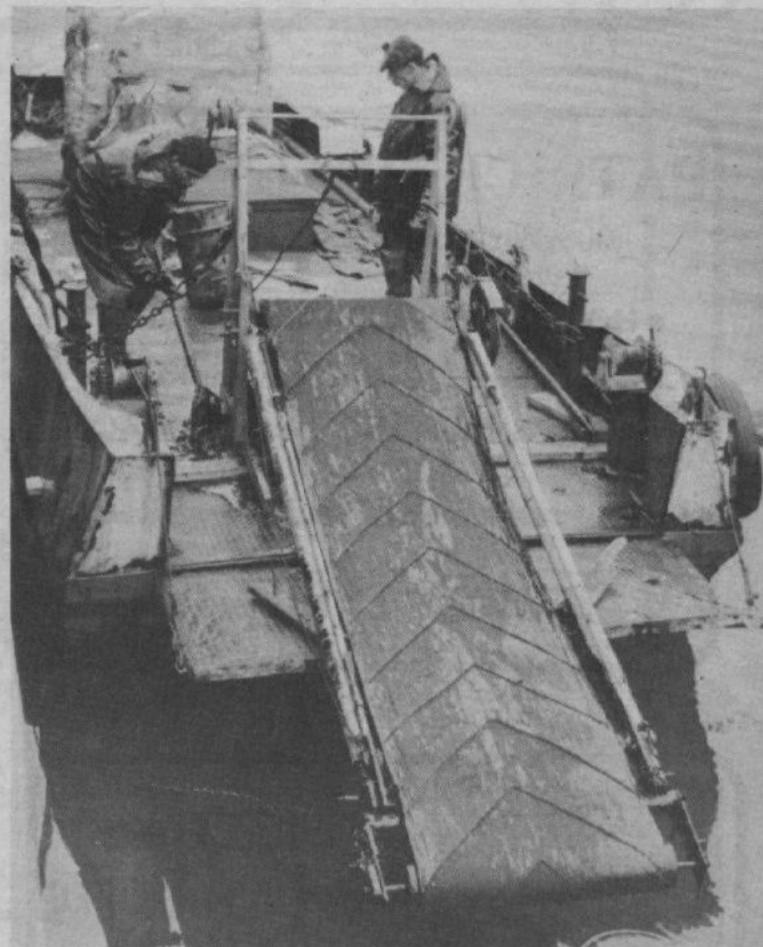
"SLICK LICKER"—Invented by a National Defence Research scientist, the famous slick-licker was one of the first practical devices for mopping up floating oil in a continuous process.
