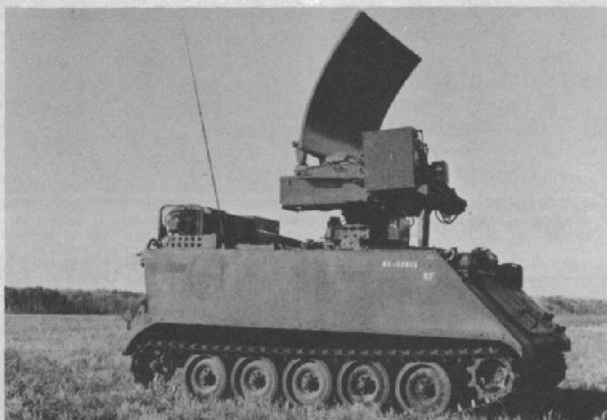
WINNIPEG, MAN., JAN. 31, 1968 — The AN MPQ Counter Mortar Radar mounted on the M113 Armoured Personnel Carrier, the "eyes" which watch an enemy shell in flight.
