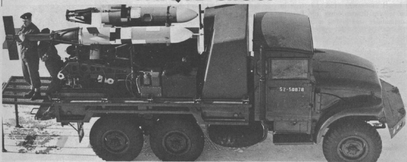
WINNIPEG, MAN., FEB. 1, 1968 — The AN USD 501 Drone, built by Canadair Ltd. Montreal, an un-manned, rocket-assisted, jet-propelled aircraft, being fitted with a solid fuel booster it lies aboard the launcher pallet.
