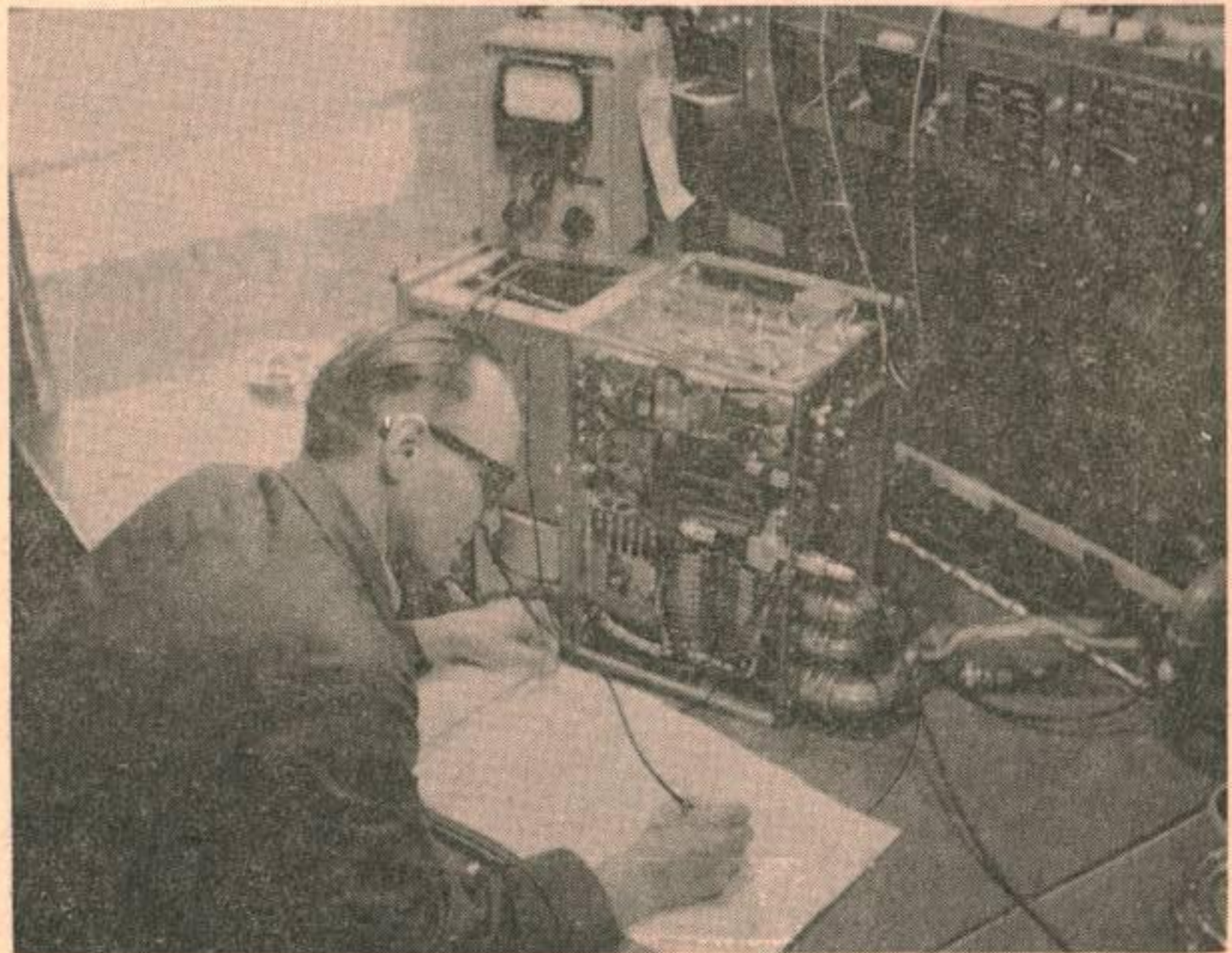
Cpl. John Paul tracking down a problem in the Remote Transmitter-Receiver Site screen-room with the aid of the UHF Test Bench and schematics.
