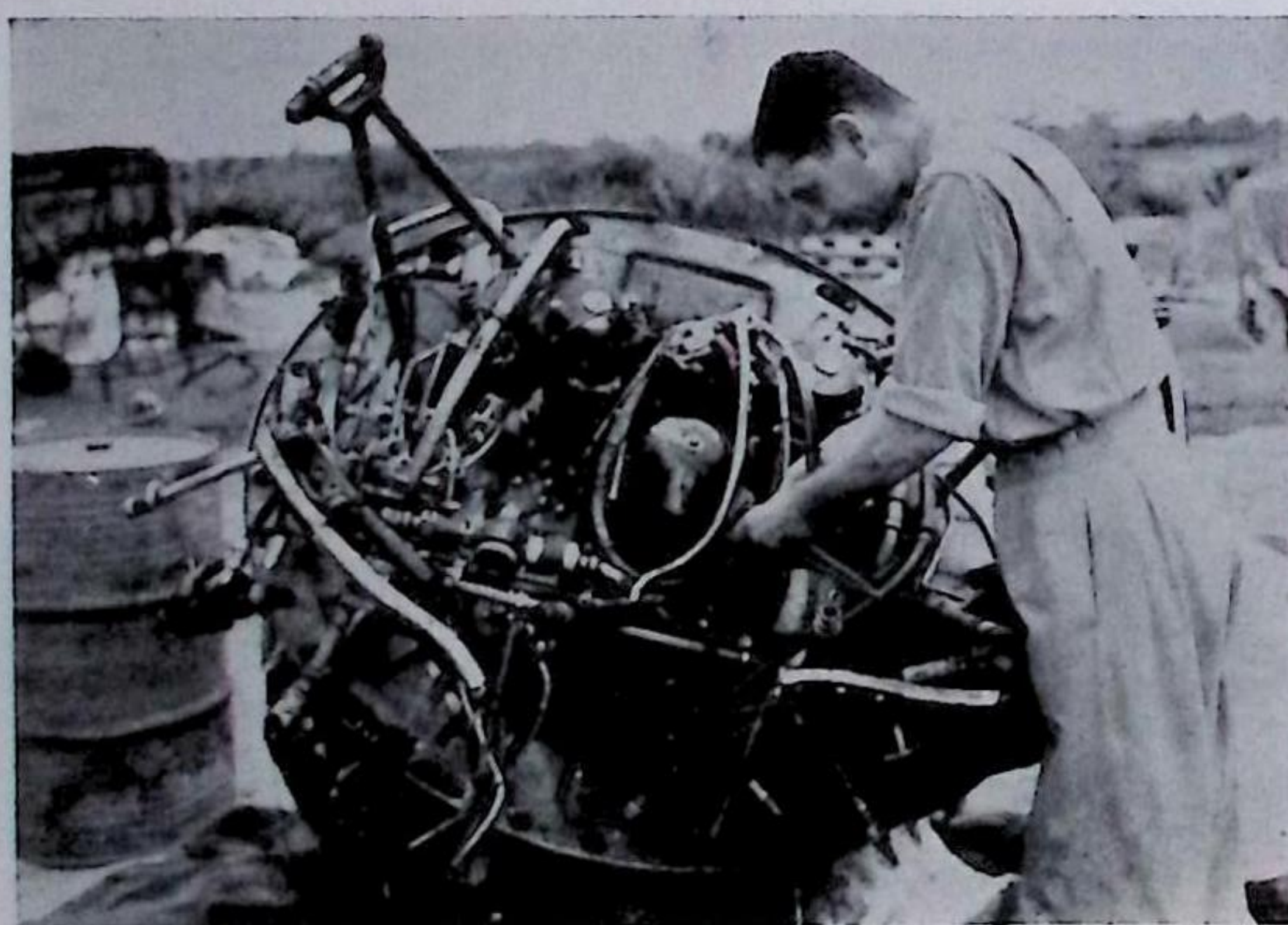
Checking the Wiring of a Dakota Motor
